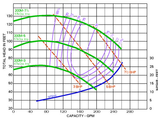
200M CENTRI-THRIFT PERFORMANCE
