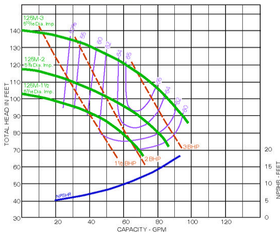
125M CENTRI-THRIFT PERFORMANCE
