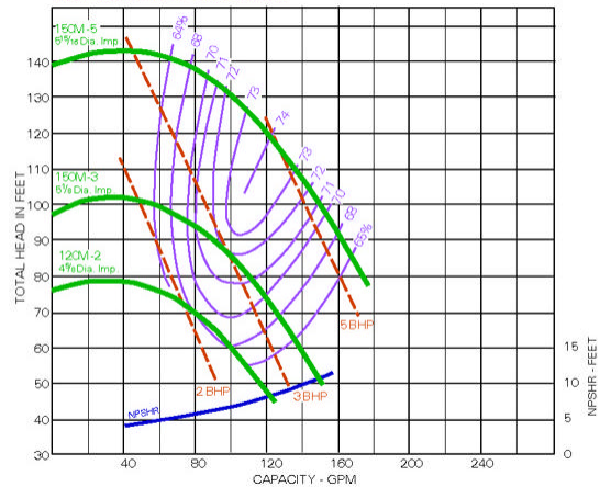
Myers M Series Centrifugal Pumps
